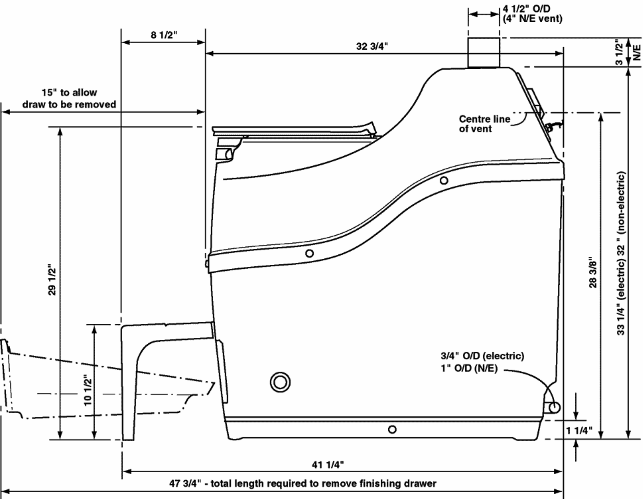
PLAN ELEVATION
