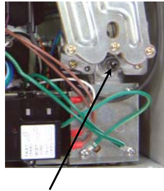
Manifold pressure tap
